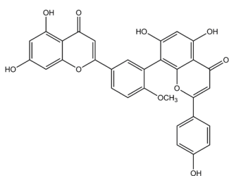
Bilobetin, (product # 83840)
