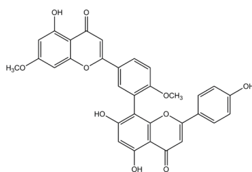
Ginkgetin, (product # 83501)
